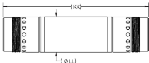
FLUIDPRO WITH PURGE PORT MODULE ONLY AIR DRYER DIMENSIONS AND MATERIALS OF CONSTRUCTION, MM (IN)
